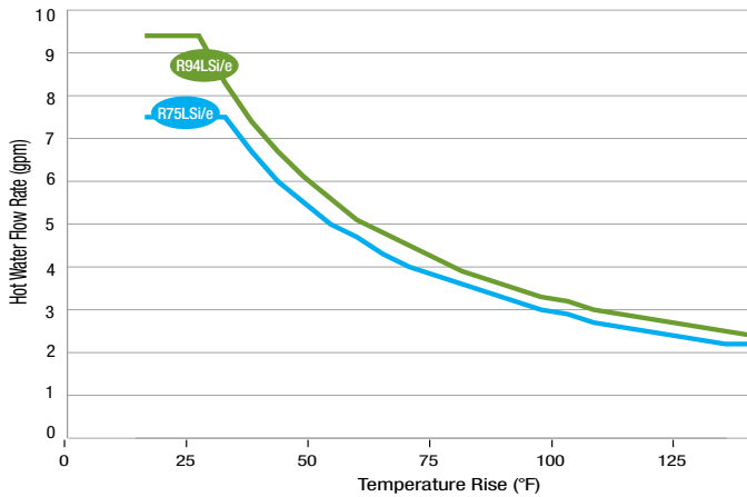
Tankless Water Heater – Maximum Flow Curves
